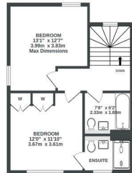
2ND FLOOR 466 sq.ft. (43.3 sq.m.) approx.
